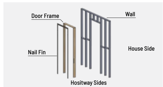
Knock down or assembled frame mounts flush to the interior of the hoistway
