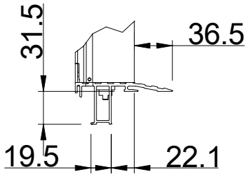
A (1:5)
