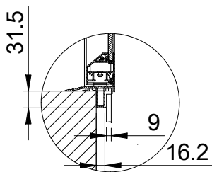
C2 (1:10)
