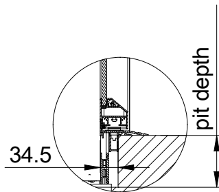
A0 (1:10)
